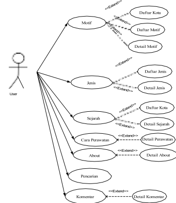
Gambar 3.1 Use Case Diagram
