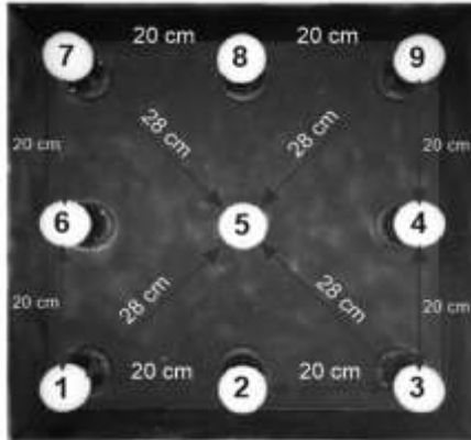
Gambar 5. (a) Jarak antar lampu
