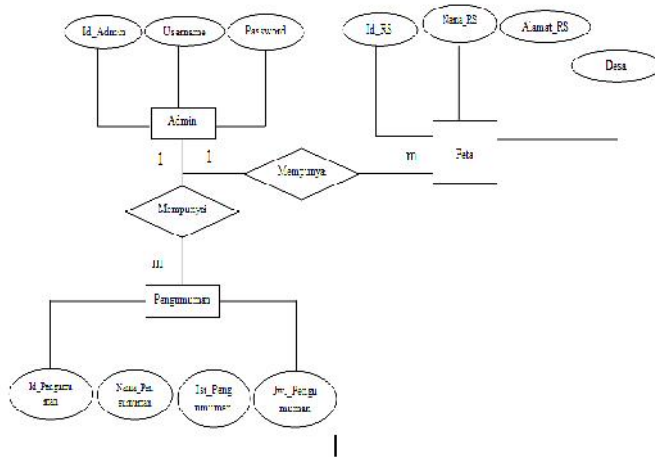
Gambar 3.3 Entity Relationship Diagram
