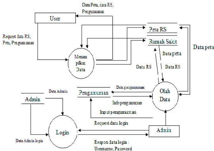
Gambar 3.3 Data Flow Diagram Level 1
